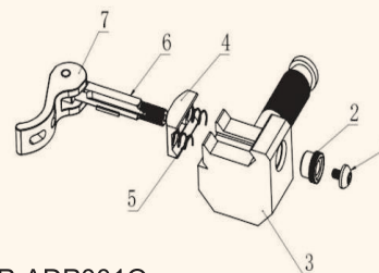
BP-ADP001Q Picatinny/Weaver, Quick-Release
