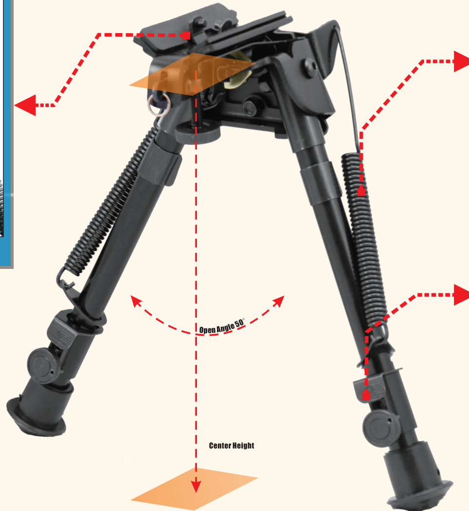
Foldable Arms with Robust External Spring Tension Control
