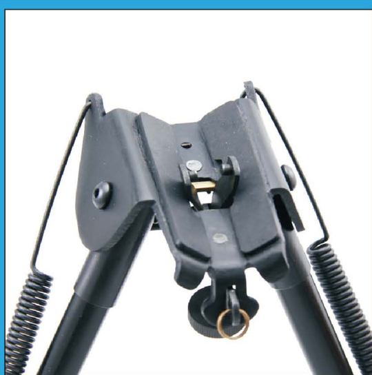
Fixed Head
